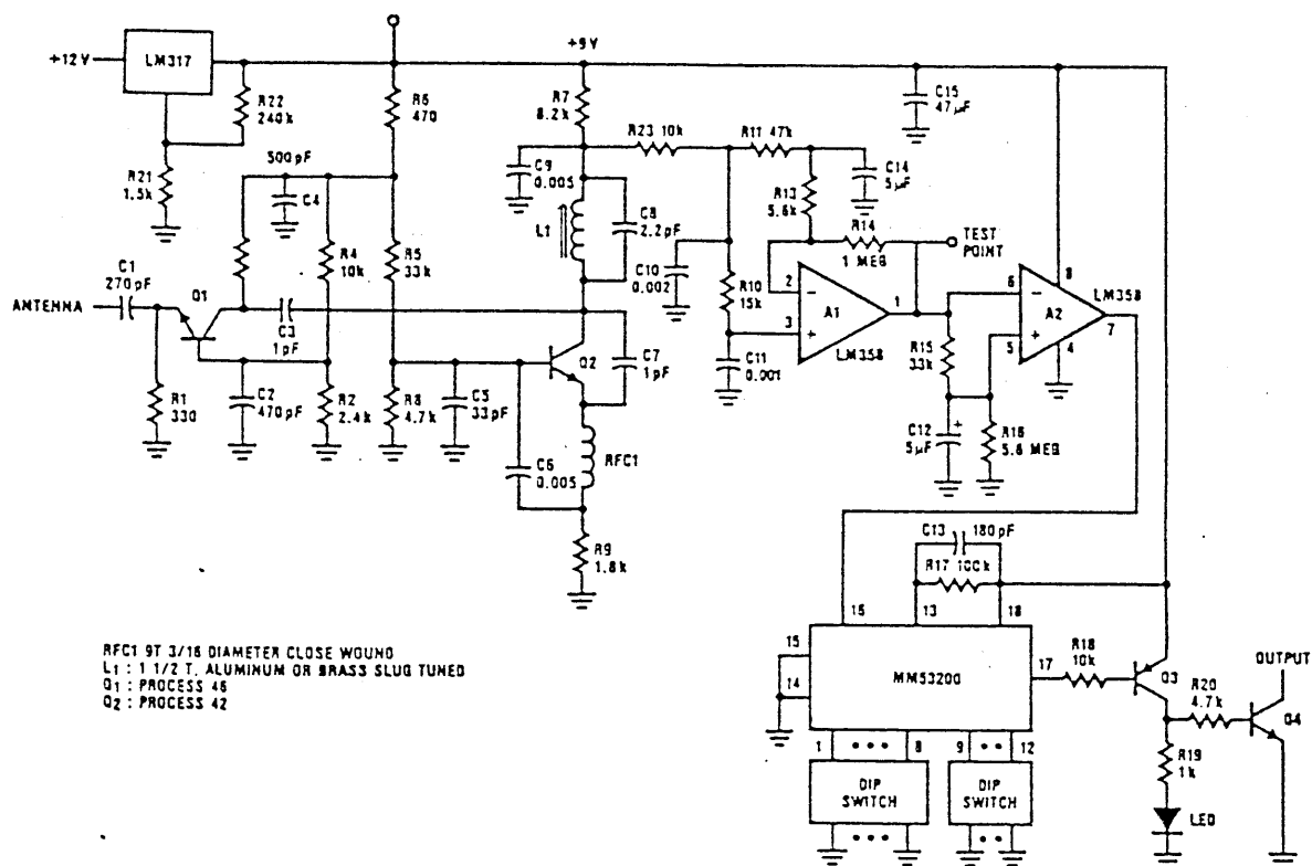
Figure 8. Remote Control Receiver.
