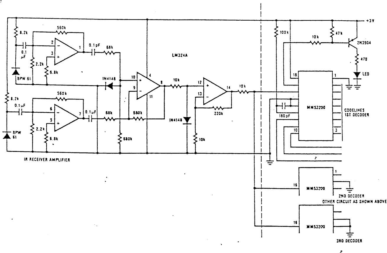
Figure 10. IR Receiver Application.
