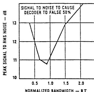
Figure 4. Signal-to-Noise vs. Normalized Bandwidth.
