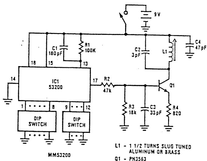
Figure 7. Remote Control Transmitter
