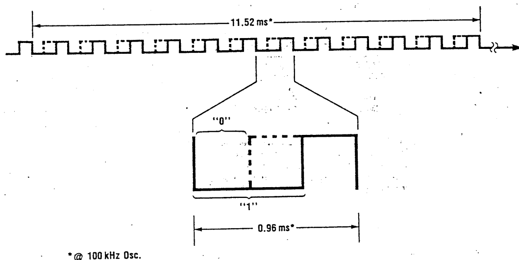
Figure 1. Output Waveform
