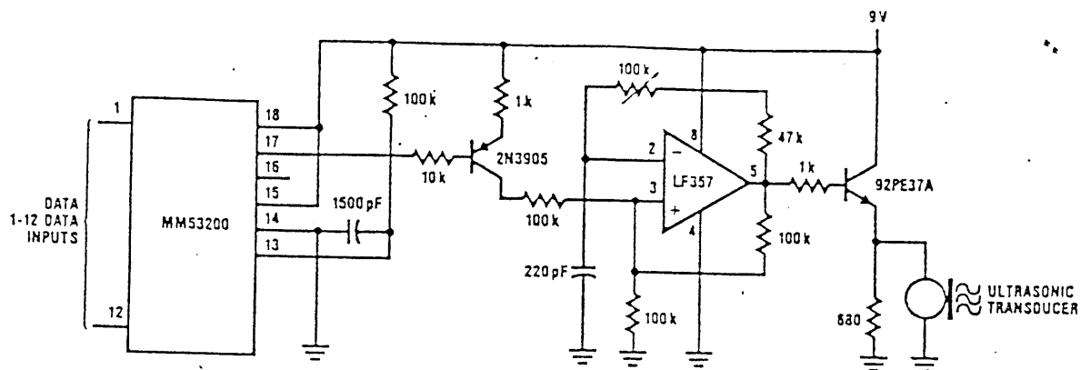
Figure 5. Ultrasonic Transmitter.
