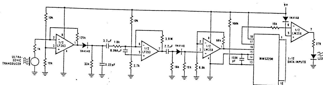
Figure 6. Ultrasonic Receiver.
