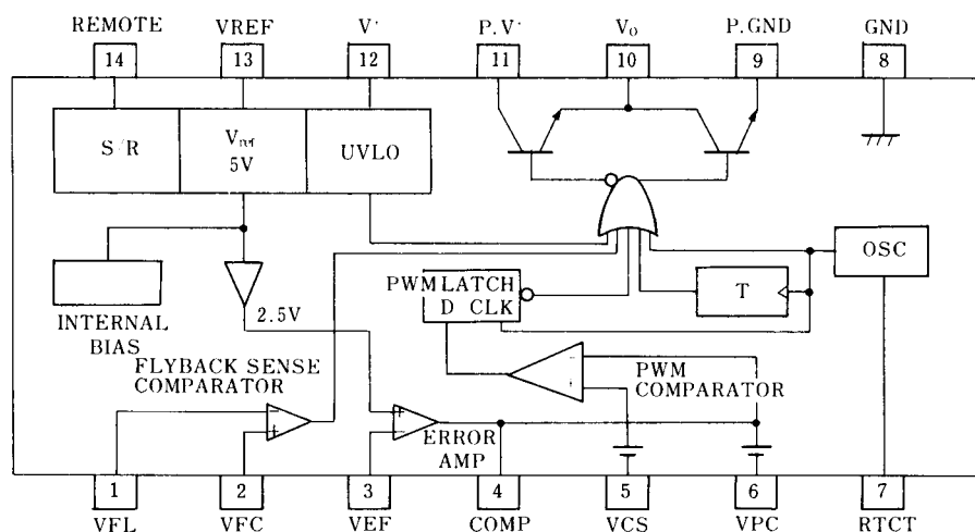
NJM2362D
