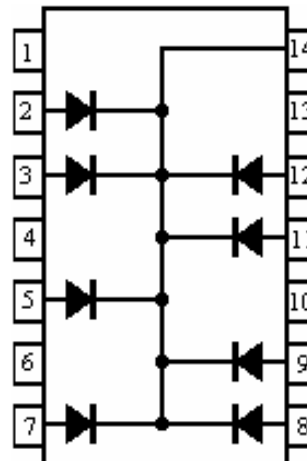
CIRCUIT CONFIGURATION
