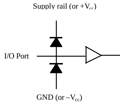
STEERING DIODE APPLICATION
