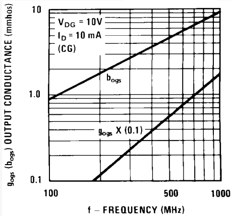
Figure 16. Output Admittance
