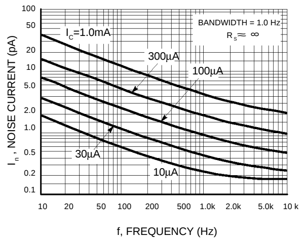
Figure 4. Noise Current
