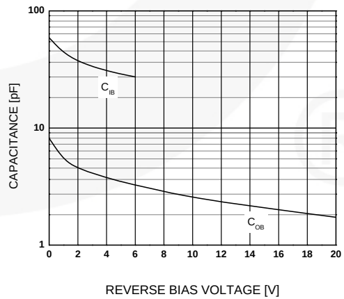
Figure 6. Collector-Base and Emitter-Base Capacitance vs. Reverse-Bias Voltage
