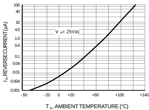
Figure 4. Leakage Current
