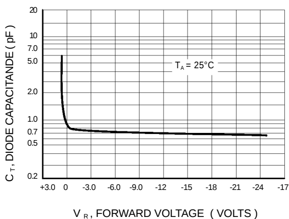
Figure 3. Diode Capacitance
