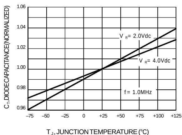
Figure 4. Diode Capacitance versus Temperature
