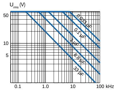
MMK7.5 ... 37.5 100/63
