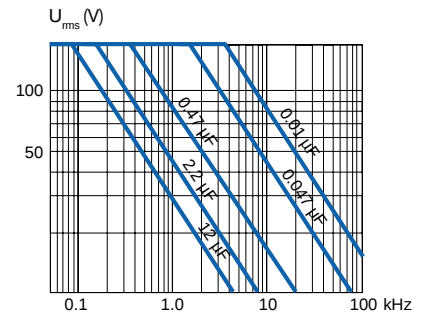
MMK7.5 ... 37.5 250/160
