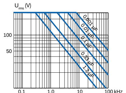
MMK7.5 ... 37.5 1000/250
