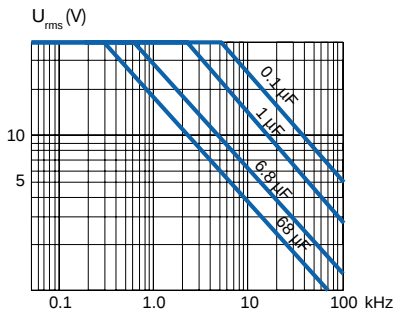
MMK7.5 ... 37.5 63/40
