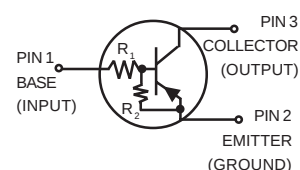
CASE 318, STYLE 6 SOT-23 (TO-236AB)
