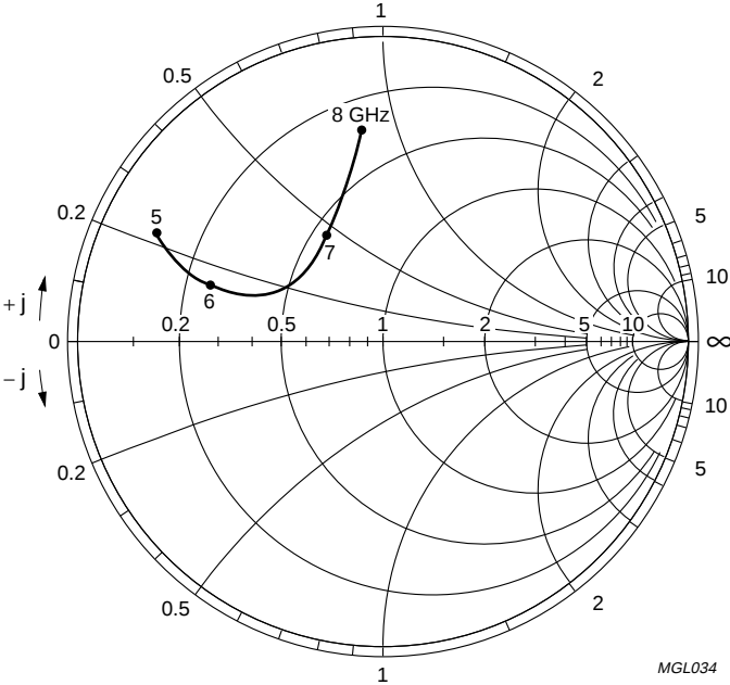
Fig.4 Base reflection coefficient
