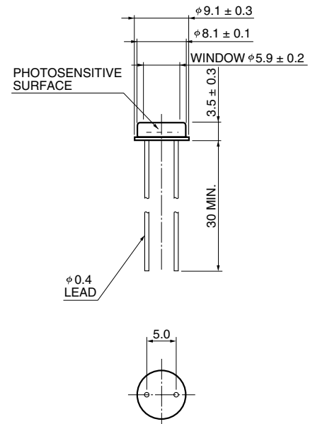
③ 8M type (TO-5)
