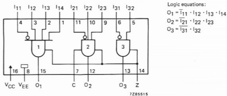
Fig. 1 Logic diagram.
