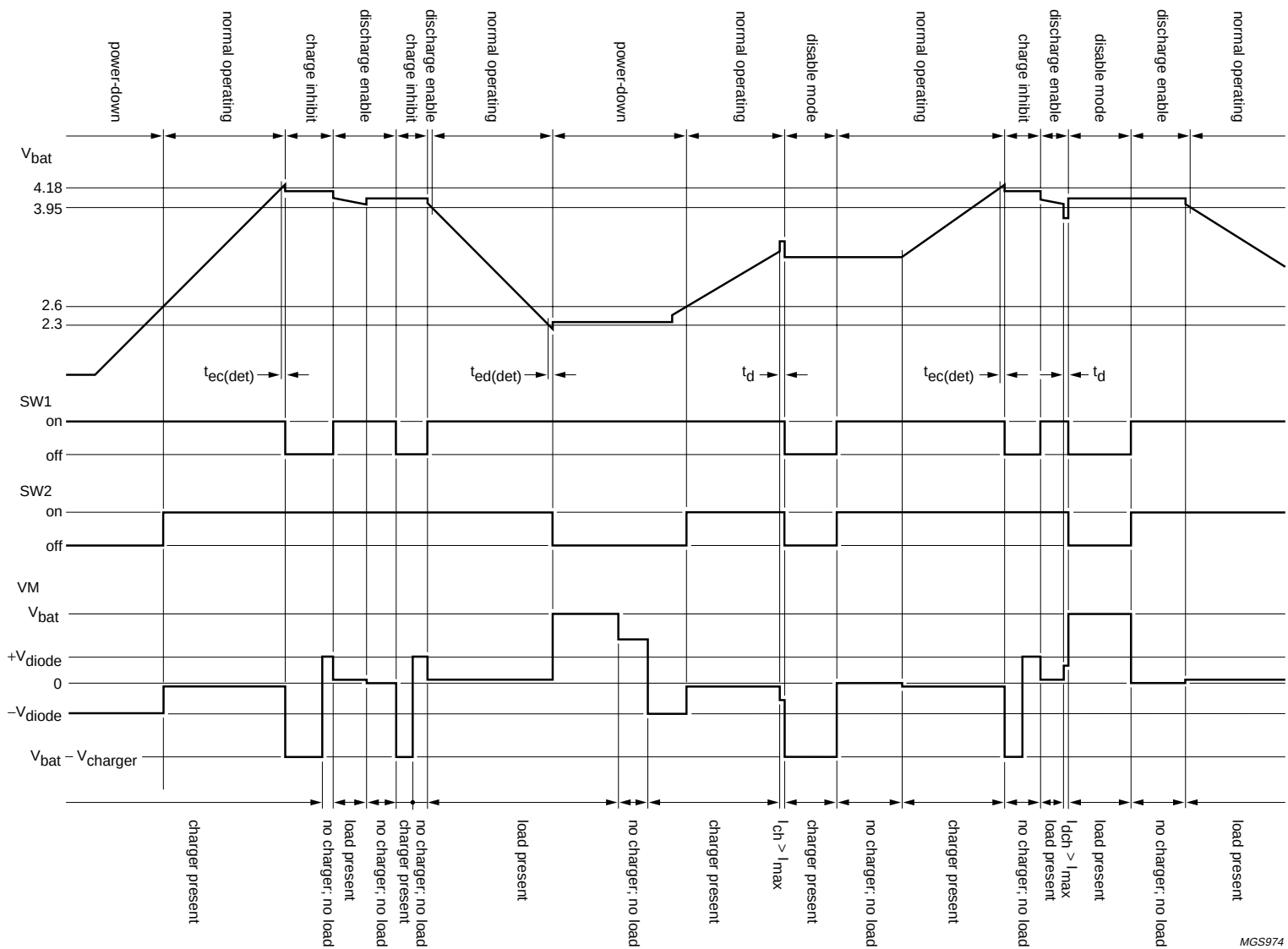
Fig.6 Timing diagram.
