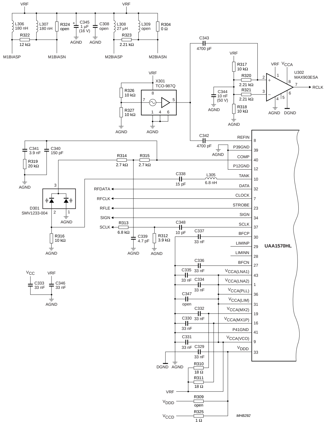
Fig.25 RF front-end circuit (continued in Fig.26).
