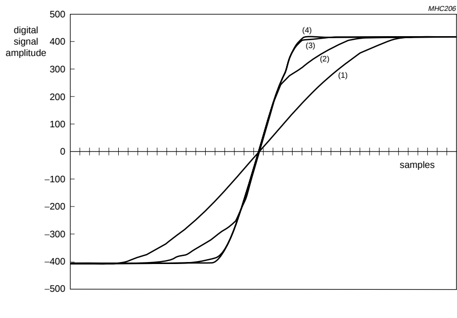
Fig.11 DCTI with variation of limit setting (gain = 7).
