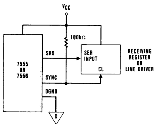
Figure 17. Serial Data Transfer
