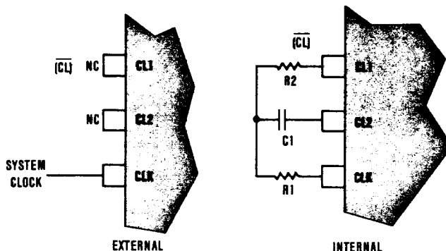
Figure 9. Clocking Configurations
