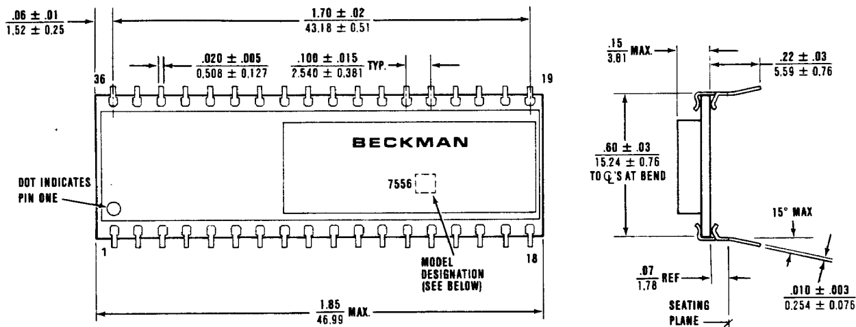
Outline Drawing—Series 7556
