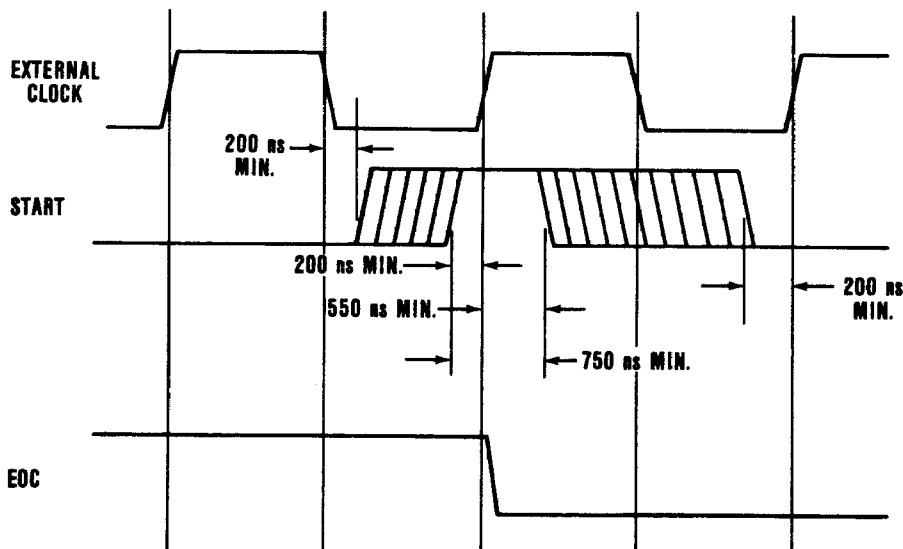
Figure 12. START Timing—External Clock
