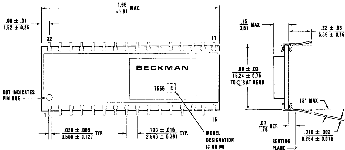
Outline Drawing—Series 7555
