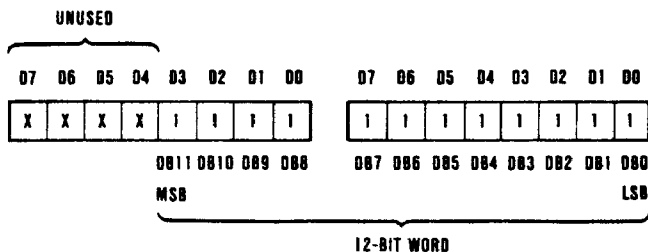
Figure 16. 12-Bit Data Format
