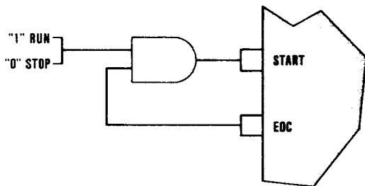
Figure 13. RUN/STOP Operation
