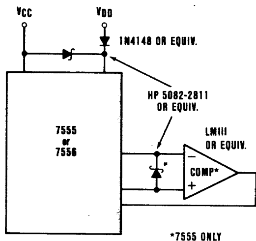
Figure 5. Diode Protection
