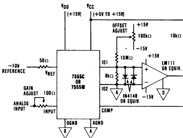
Figure 18. Unipolar Operation (7555)
