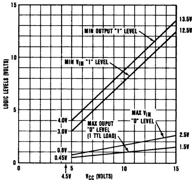
Figure 7. Input/Output Logic Levels
