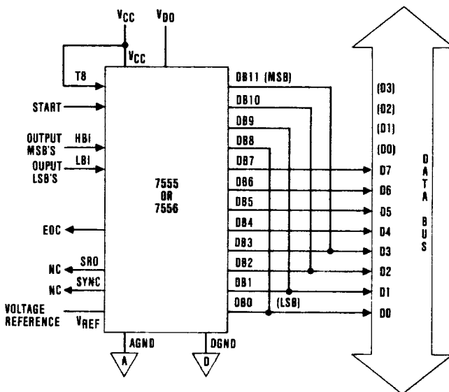
Figure 15. 12-Bit Output to 8-Bit Data Bus
