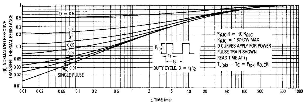
Figure 10. Thermal Response
