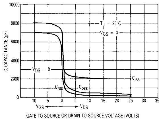
Figure 11. Capacitance Variation
