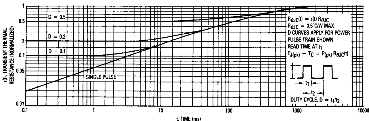
Figure 10. Thermal Response
