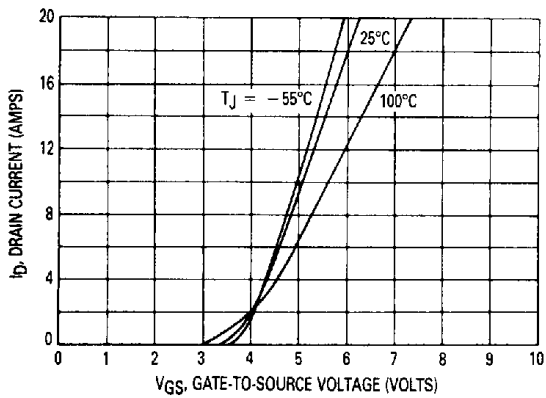
Figure 3. Transfer Characteristics
