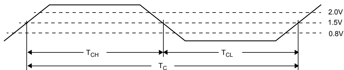
Figure 5. Timing Waveform
