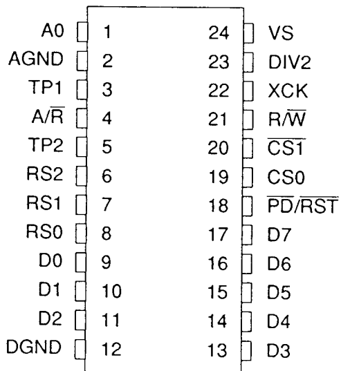
24-Pin DIP
