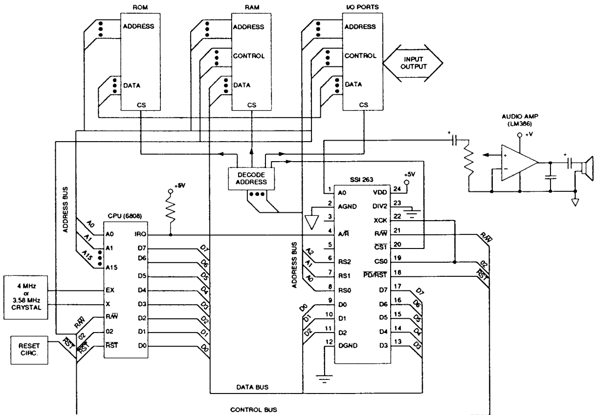
FIGURE 3: Typical Microprocessor Implementation
