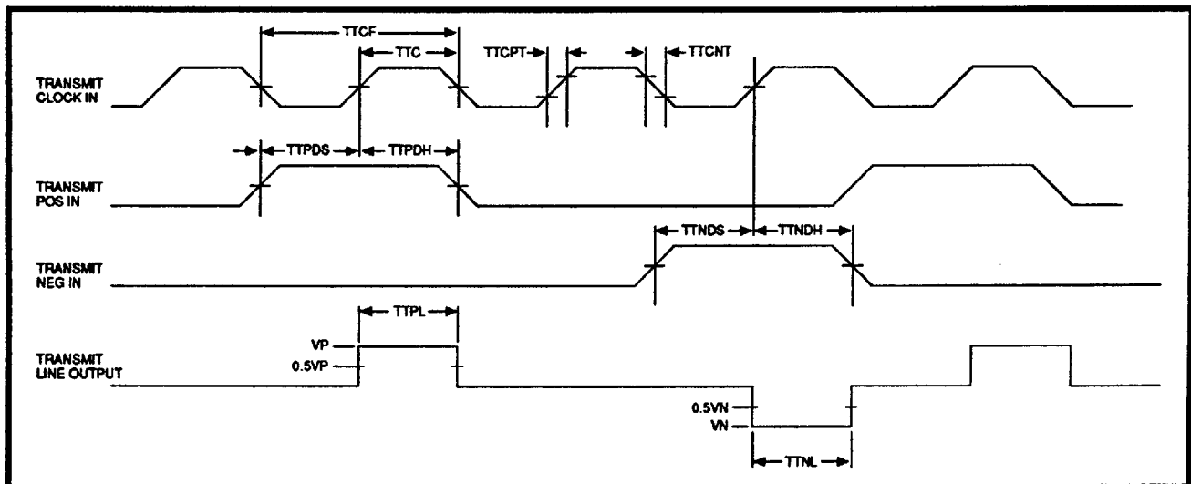
FIGURE 3: Transmit Waveforms
