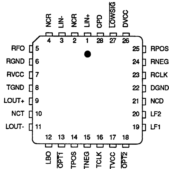
28-Pin PLCC
