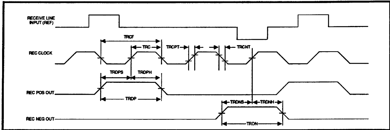
FIGURE 2: Receive Waveforms
