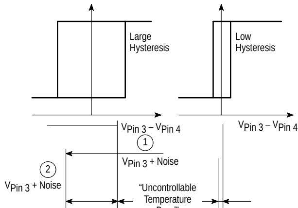
Figure 5. Effects of Inputs Comparator Hysteresis
