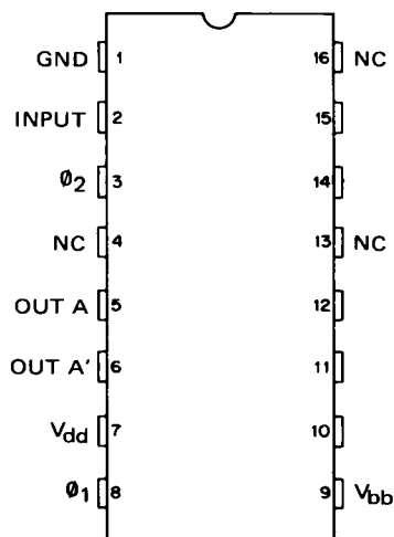
Figure 15. Pin Configuration, SAD-512.
