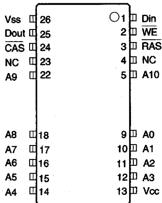
26/20-pin TSOP TYPE ( II ) Reverse Bend ( 300 mil ) P26/20TP-2A-R
