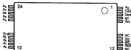
20/24-pin TSOP TYPE ( 1 ) Reverse Bend ( 6 × 16mm ) P24TV-5B4-R
