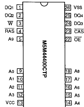
Outline 26P3Z-E(300mil TSOP)
