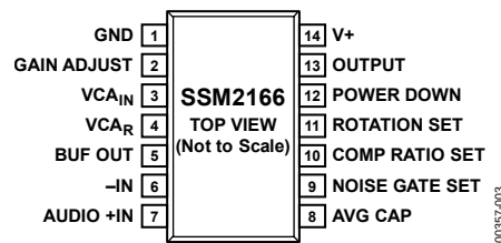
Figure 3. Pin Configuration
