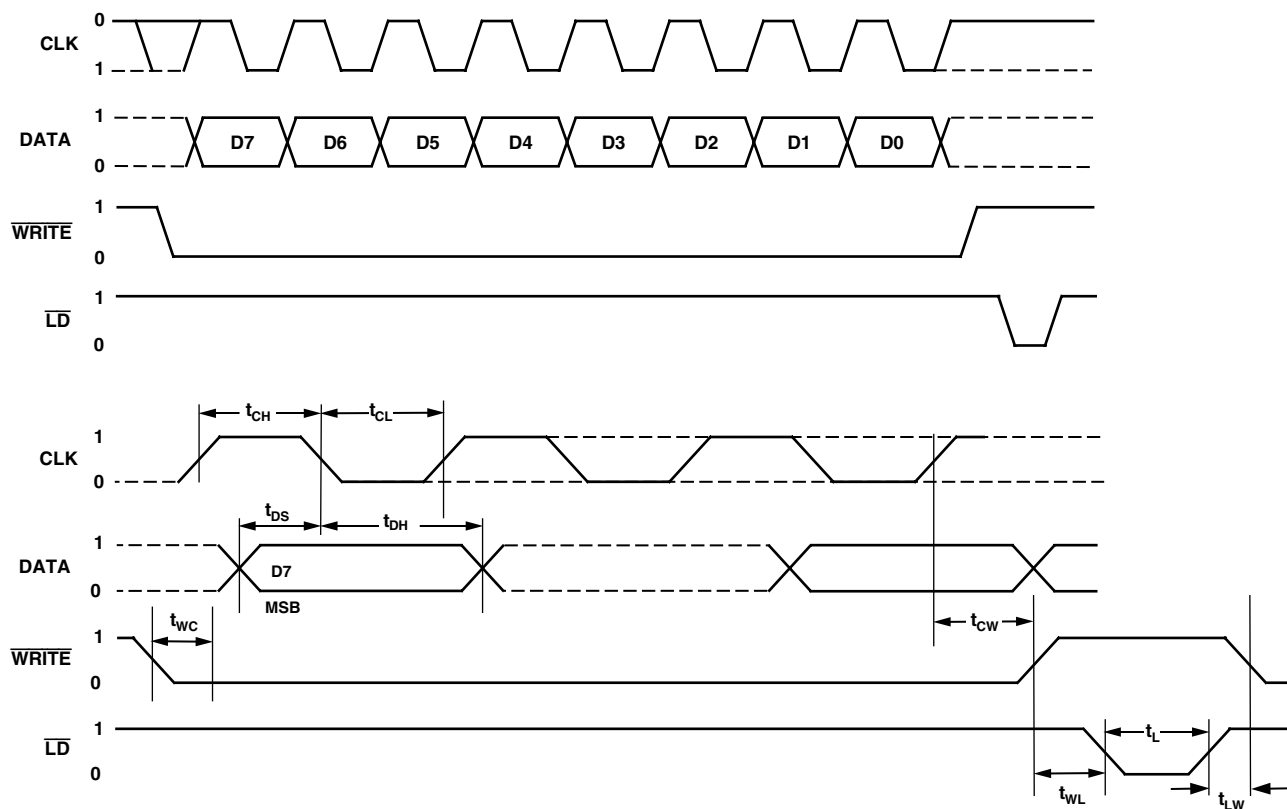
Figure 1. Timing Diagrams
