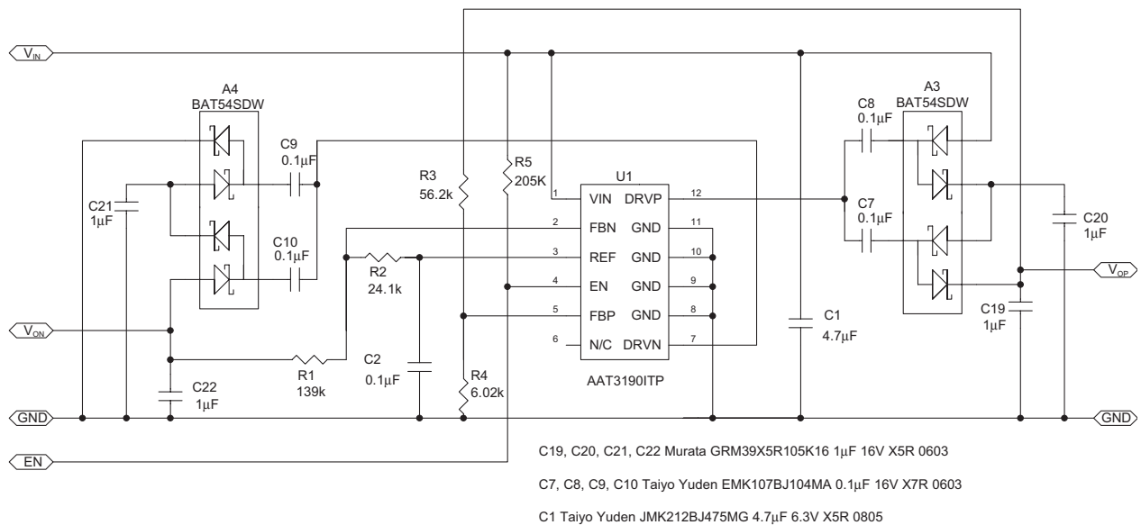
Figure 5: AAT3190 Evaluation Board Schematic (shown with two stages) V_{OP} = 12V , V_{ON} = -7V .
