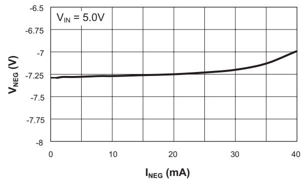
Negative Output Voltage vs. Load Current ( T_A = 25^{\circ}\text{C} )
