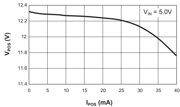
Positive Output Voltage vs. Load Current ( T_A = 25^{\circ}\text{C} )
