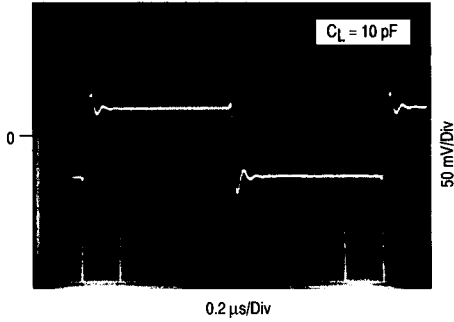
Figure 24. Small-Signal
