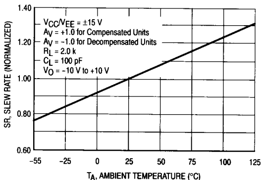
Figure 23. Normalized Slew Rate versus Temperature
