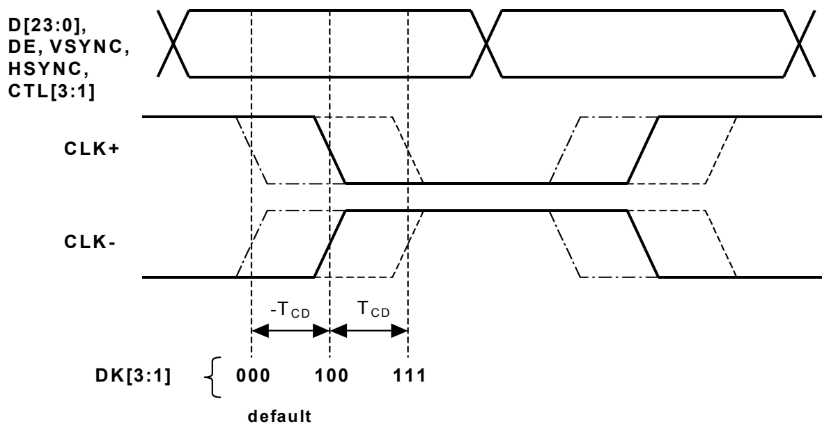
Figure 12. SiI 164 Data De-skew Feature Timing
