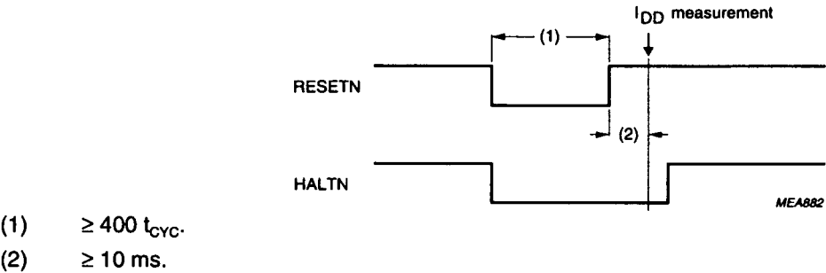
Fig.51 I_{DD} measurement.
