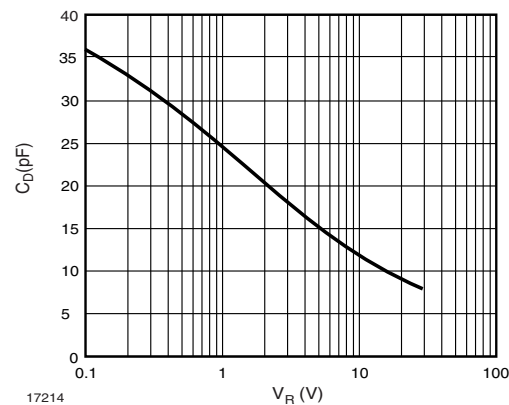
Figure 4. Diode Capacitance vs. Reverse Voltage
