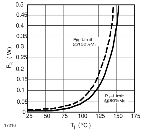
Figure 6. Max. Reverse Power Dissipation vs. Junction Temperature
