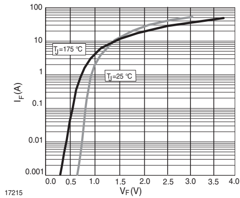
Figure 5. Typ. Forward Current vs. Forward Voltage
