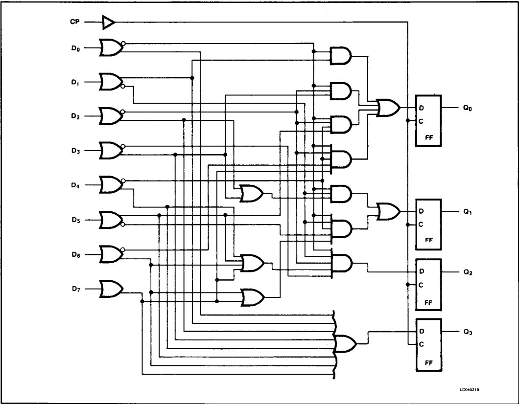
LOGIC DIAGRAM
