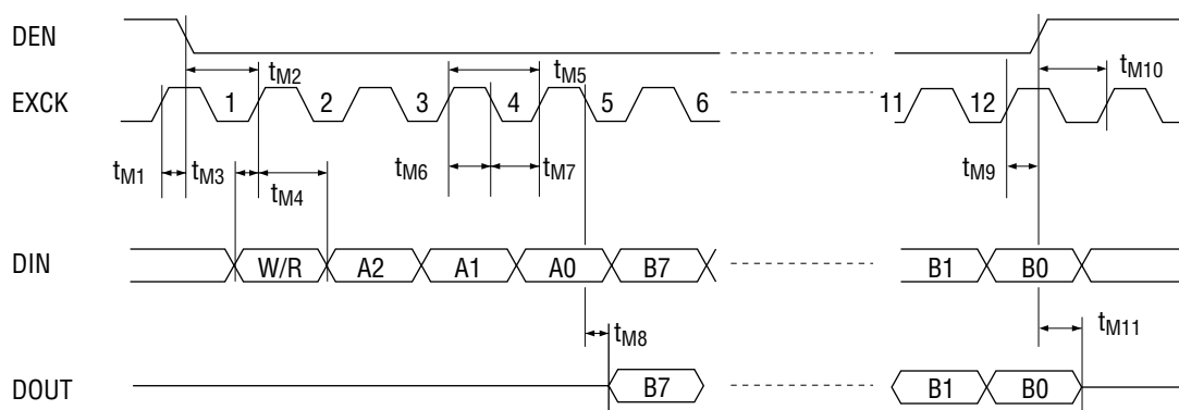
Figure 8 Serial Control Port Interface
