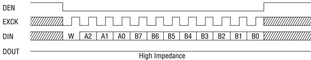
(a) Write Data Timing Diagram
