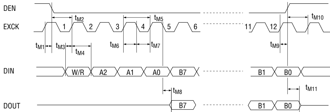
Figure 5 MCU Interface
