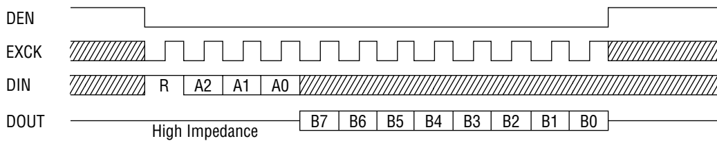
(b) Read Data Timing Diagram
