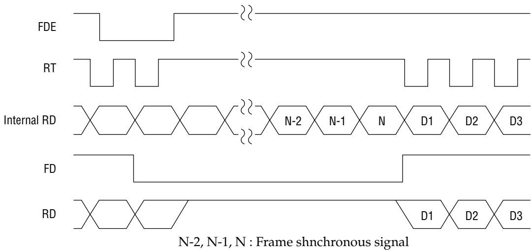
Figure 3 Receive Signal Timing
