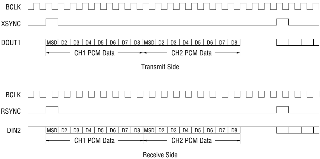
Figure. 2 Timing Diagram in the Serial Mode (CHPS = 0)
