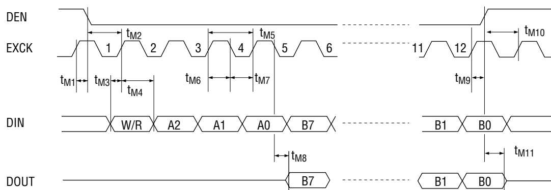
Figure 5 MCU Interface
