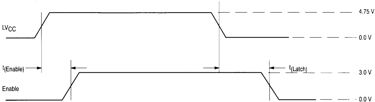
Figure 2. Timing Requirements
