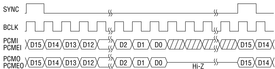
(a) 16-bit linear coding format timing (normal sync)
