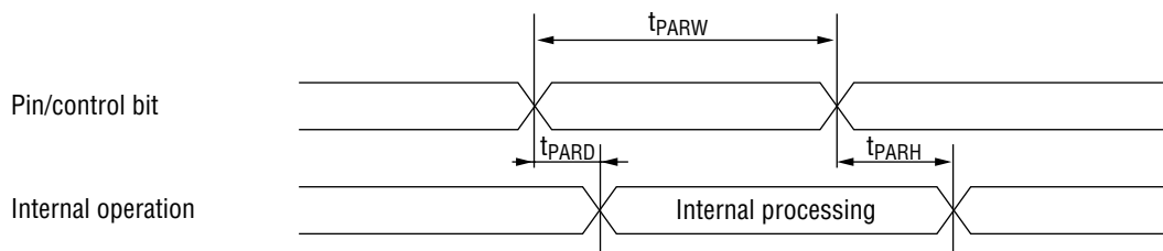
Control Timing
