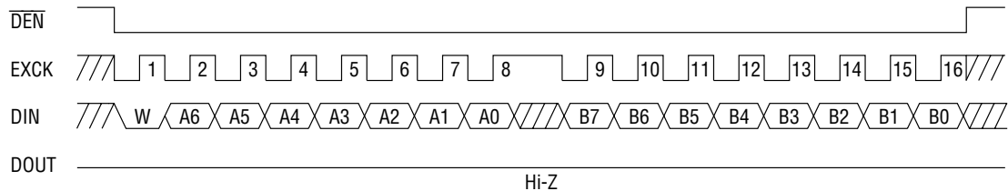
(a) Data Write Timing 1 (8-Bit MCU)
