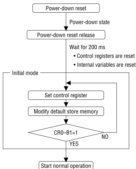
Figure 5 Initial Mode Flowchart
