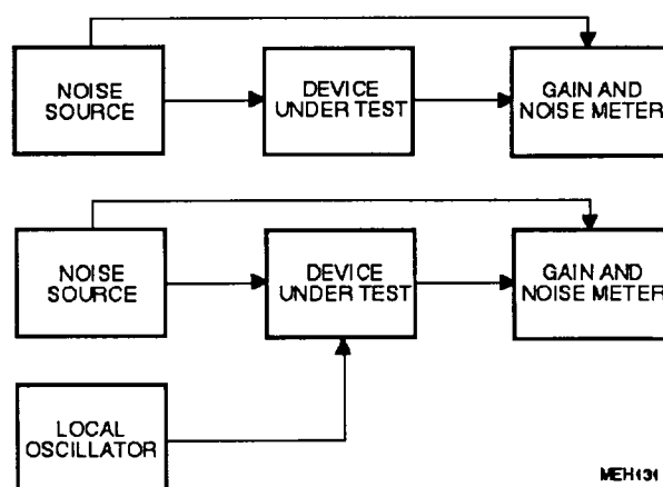
Fig.4 Noise measurements.
