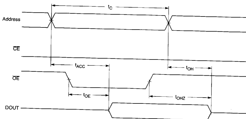
Figure 1. Read Cycle 1
