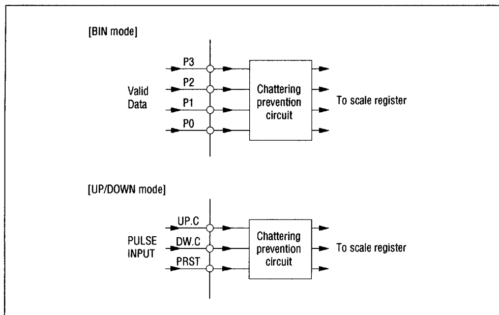
Figure 4 Scale Control Circuit
