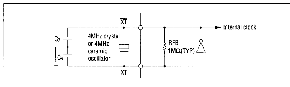
Figure 5 Oscillation Circuit
