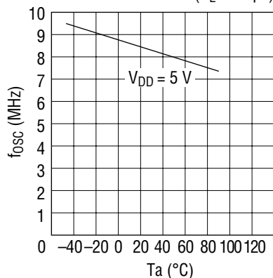
Maximum Clock Frequency ( f_{OSC} ) vs. Temperature ( T_a )
