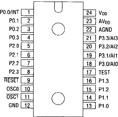
24-Pin Plastic DIP
