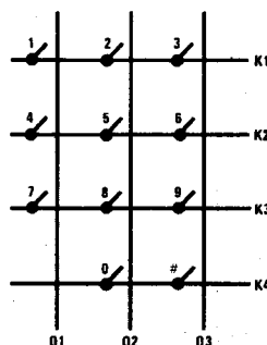
FIGURE 7. Keypad Matrix
