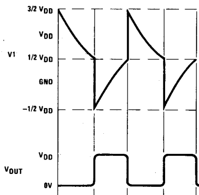
FIGURE 3. Three Gate Oscillator and Waveforms
