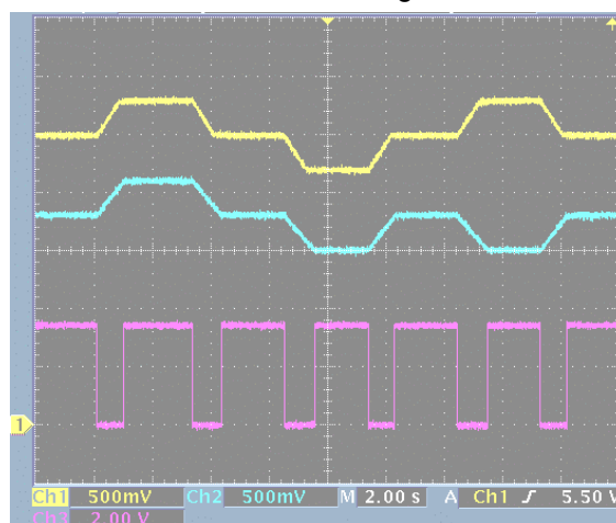
Figure 5 – SMM205 margin example. The nominal setting for channel 1 and 2 is 2.5V and 1.8V. The device margins the DC/DC converters from nominal to high (2.8V and 2.1) then to nominal, then to low (2.3V and 1.5V), then to nominal, then to channel 1 high and channel 2 low, and then back to nominal. The READY signals goes low when margining and high when complete.
