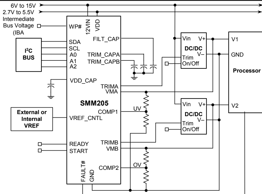
Figure 1 – Applications Schematic showing the SMM205 ADOC actively control the DC output level of 2 DC/DC Converters as well as provide margin control. The SMM205 can operate over a wide supply range
