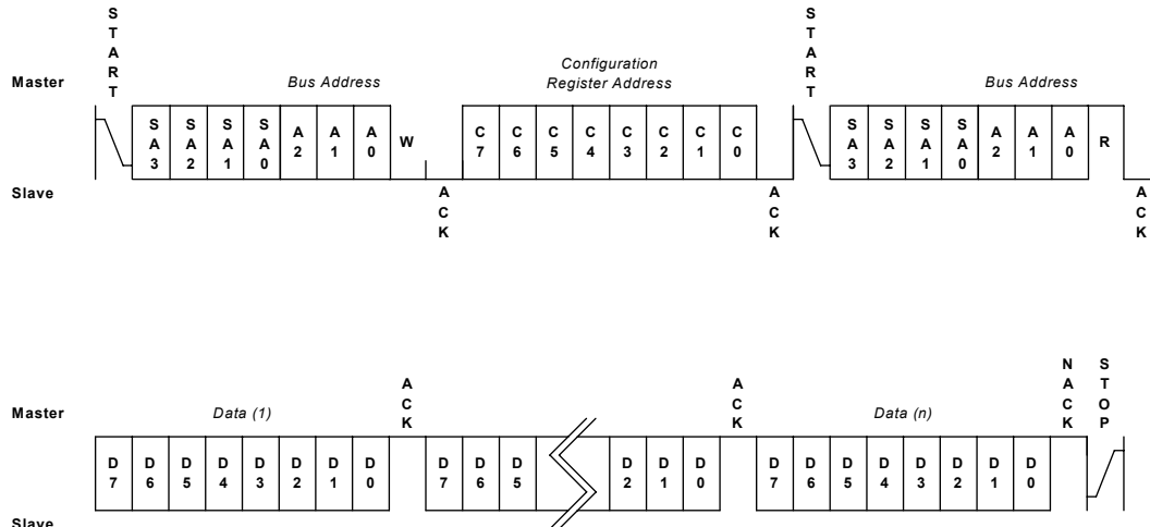
Figure 15 - General Purpose Memory Read
