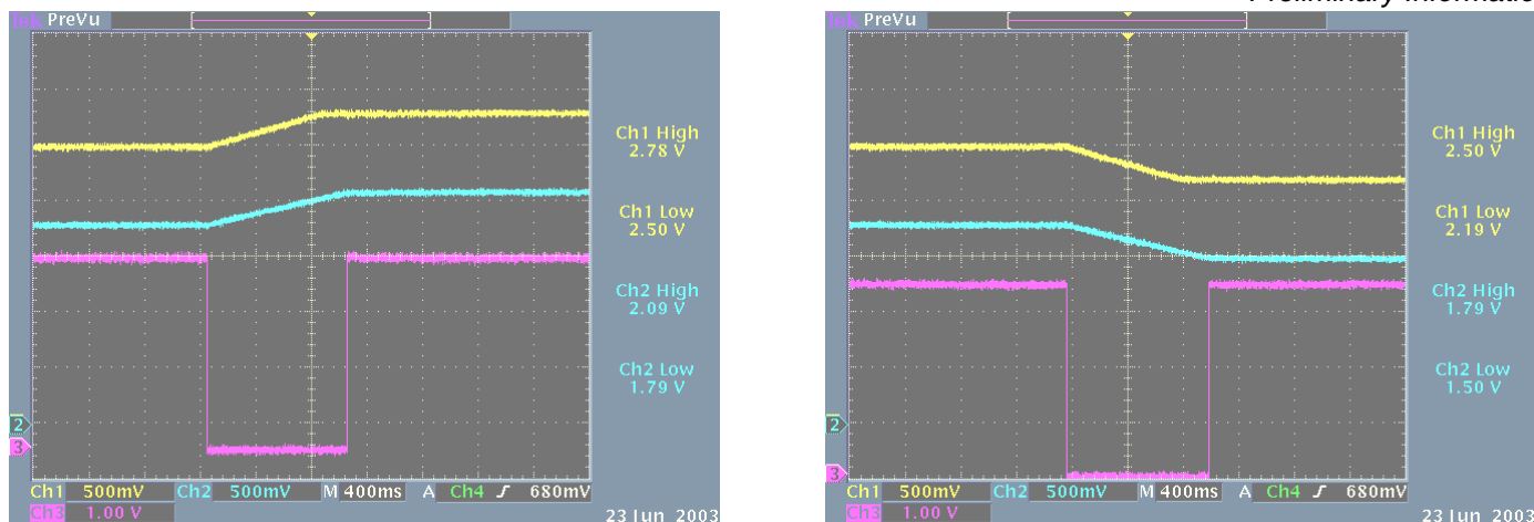
Figure 2 – Example Power Supply Margining using the SMM205. The waveform on the left is margin nominal to high from 2.5V to 2.8V and 1.8V to 2.1V. The waveform on the right is margin nominal to low from 2.5V to 2.2V and 1.8V to 1.5V. The bottom waveform is the READY signal indicating when margining is complete.
