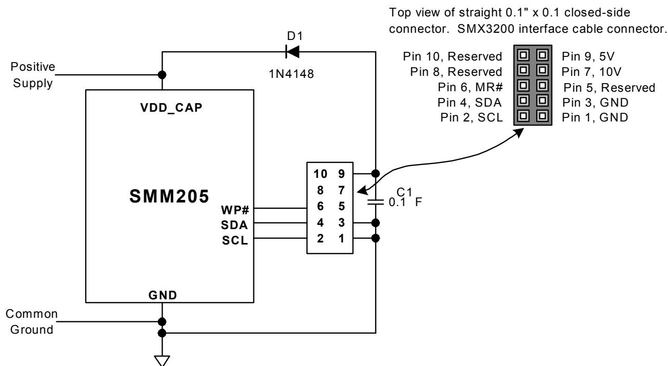
Figure 8– SMX3200 Programmer I 2 C serial bus connections to program the SMM205. The SMM205 has a Write Protect pin (WP#) which, when asserted, prevents writing to the configuration registers and EE memory. In addition, there is a configuration register lock bit which, once programmed, does not allow the configuration registers to be changed.
