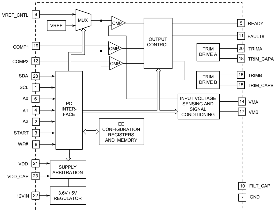
Figure 3 –Block Diagram.
